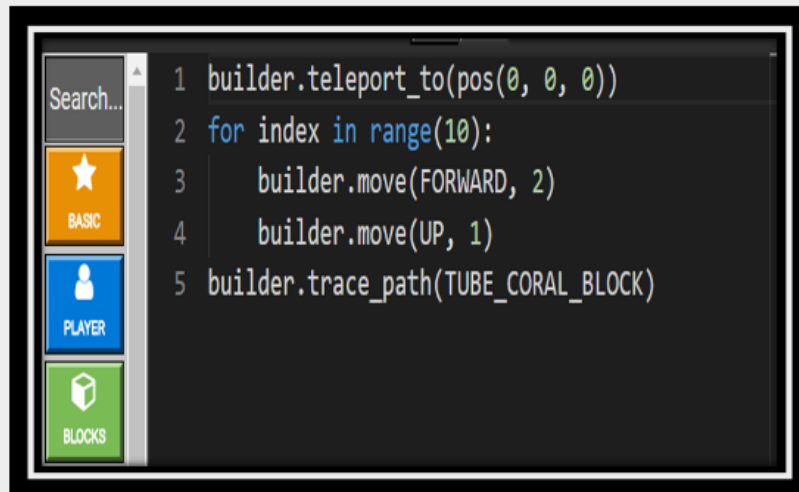
Using python
