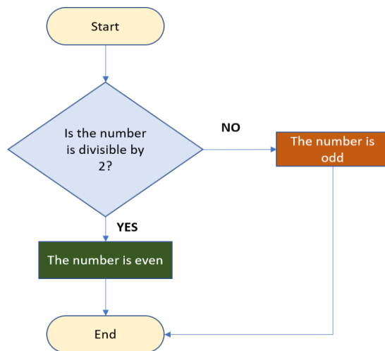
Fig 1.1 Understanding if-else
